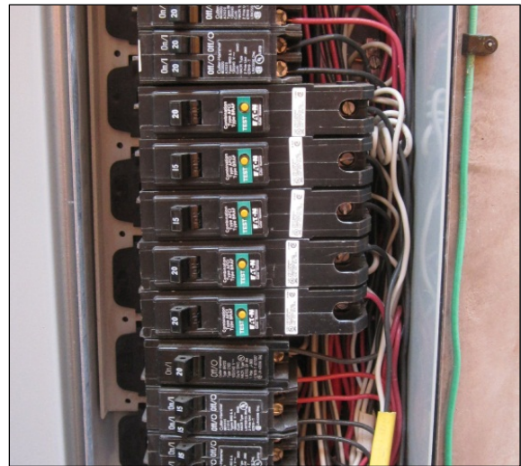
Figure 7 – Eaton AFCIs
